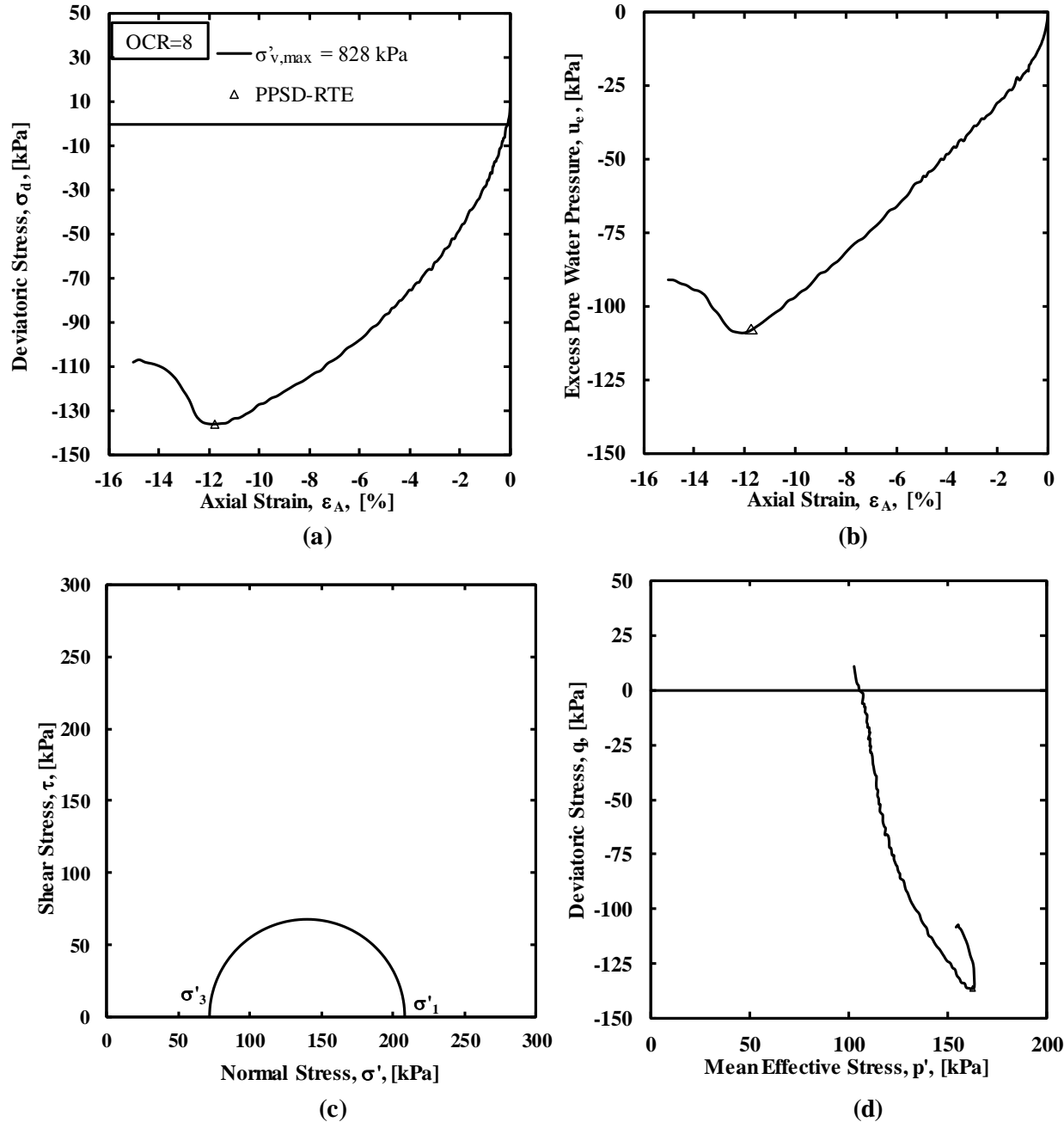
Figure A.50. a) Deviatoric stress as a function of axial strain, b) excess pore water pressure as a function of axial strain, c) Mohr circle, and d) Cambridge p-q stress path for the RTE test at OCR=8 and \sigma'_{v,max}=828 kPa.
