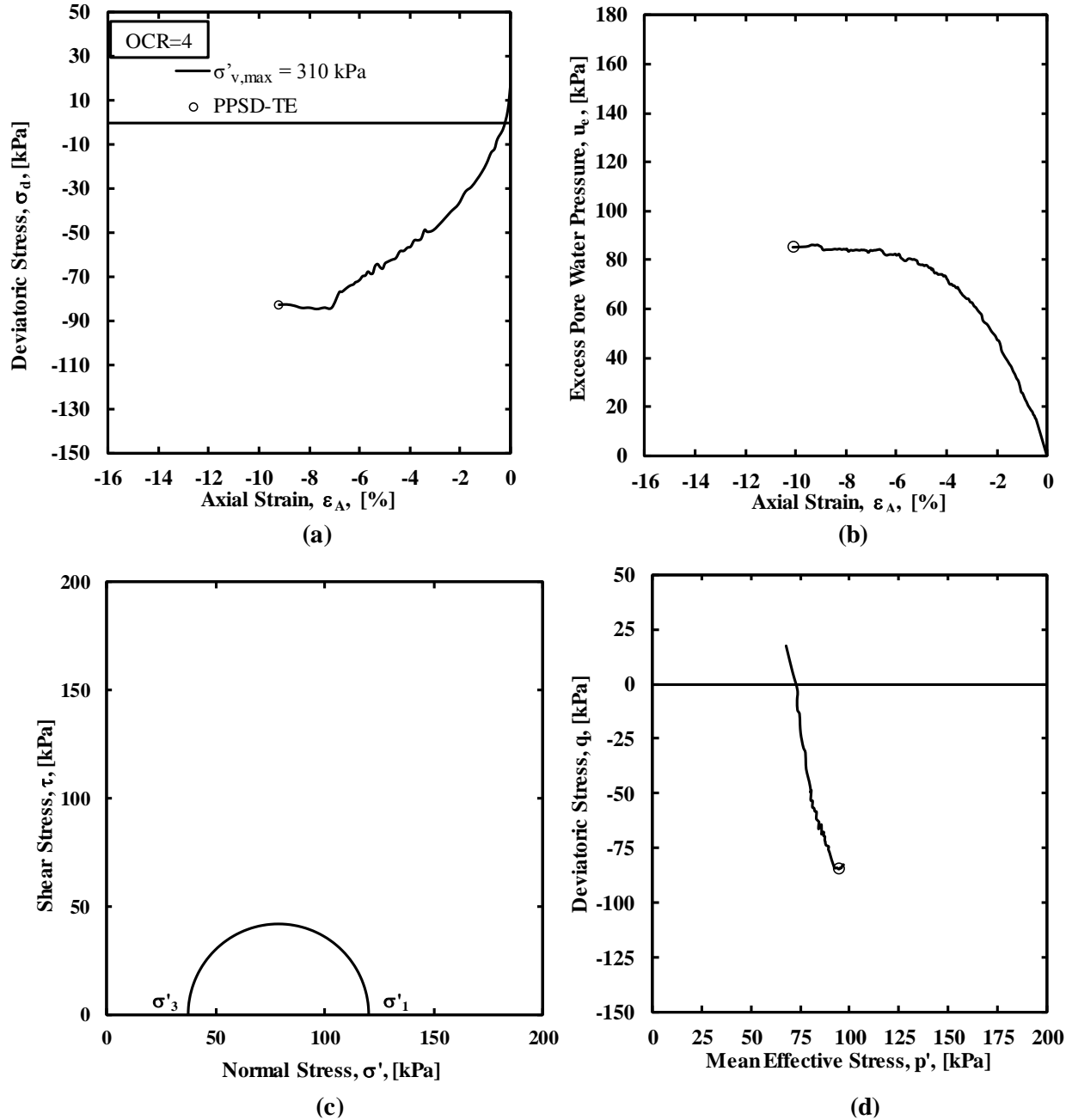
Figure A.33. a) Deviatoric stress as a function of axial strain, b) excess pore water pressure as a function of axial strain, c) Mohr circle, and d) Cambridge p - q stress path for the TE test at OCR=4 and \sigma'_{v,max}=310 kPa.
