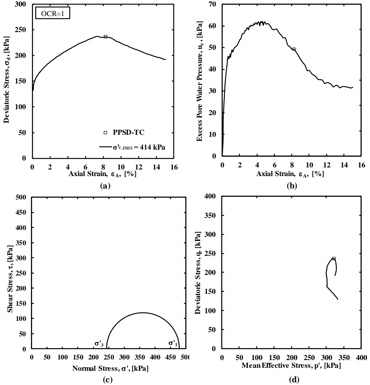
Figure A.4. a) Deviatoric stress as a function of axial strain, b) excess pore water pressure as a function of axial strain, c) Mohr circle, and d) Cambridge p - q stress path for the TC test at OCR=1 and \sigma'_{v,max}=414 kPa.
