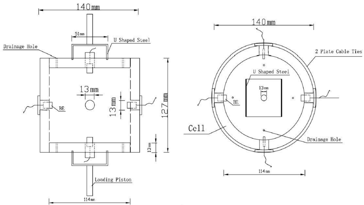
Figure 2.15. Bender elements installed in the vertical and horizontal directions within an oedometer device (after Kang et al. 2014).
