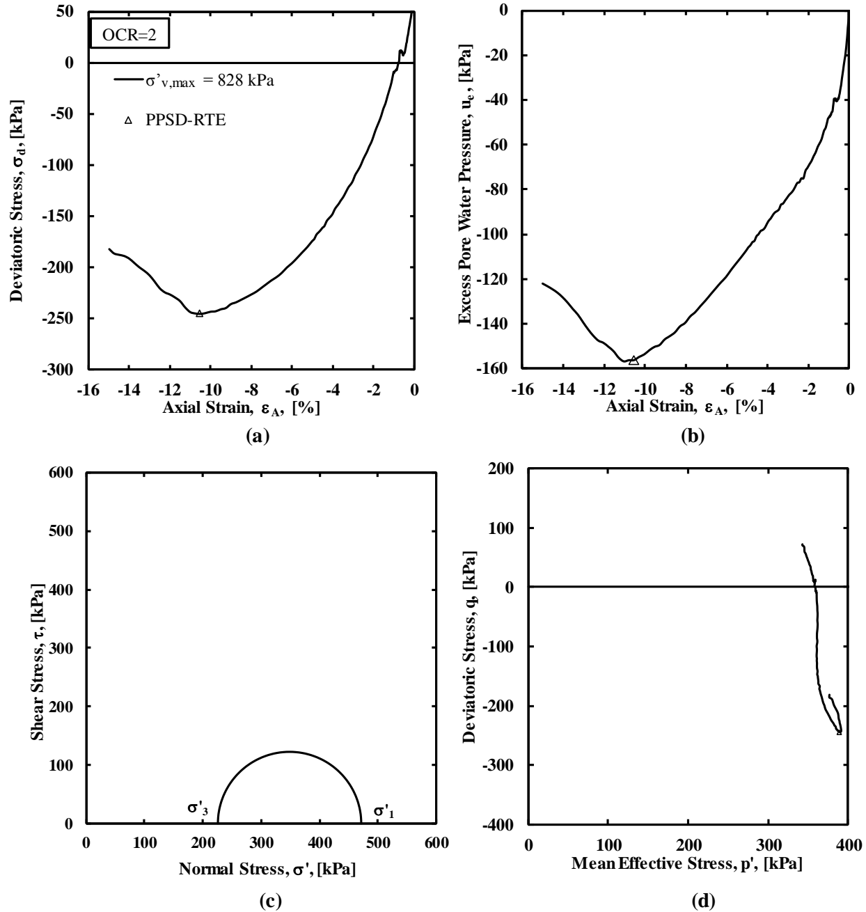
Figure A.44. a) Deviatoric stress as a function of axial strain, b) excess pore water pressure as a function of axial strain, c) Mohr circle, and d) Cambridge p - q stress path for the RTE test at OCR=2 and \sigma'_{v,max}=828 kPa.
