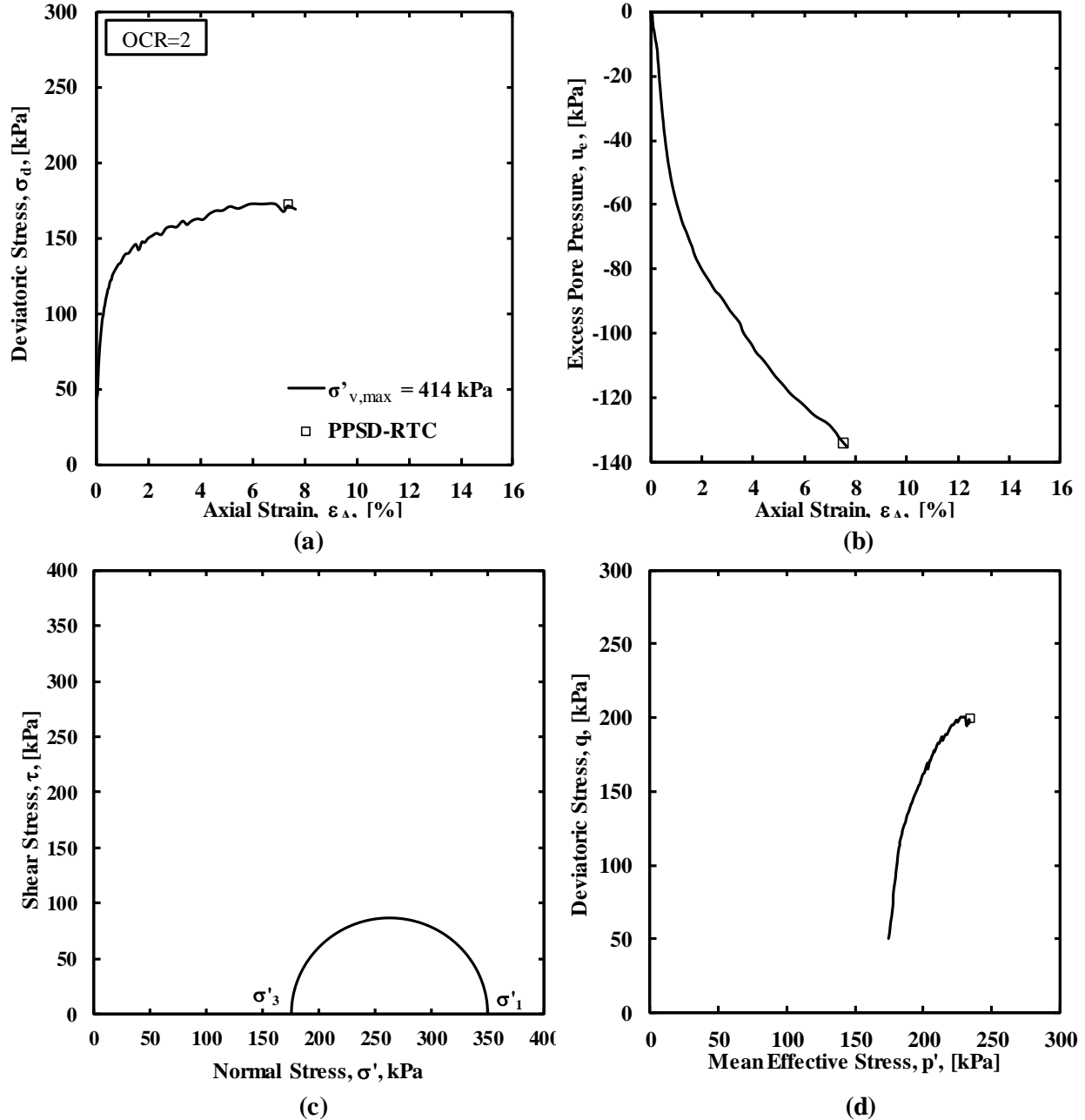
Figure A.19. a) Deviatoric stress as a function of axial strain, b) excess pore water pressure as a function of axial strain, c) Mohr circle, and d) Cambridge p-q stress path for the RTC test at OCR=2 and \sigma'_{v,max}=414 kPa.
